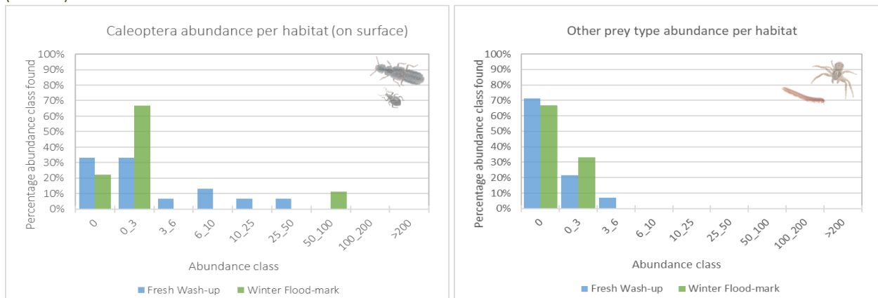
Figure 33: Graph showing the percentage of samples each abundance class of Coleoptera was found for each habitat. n = 21
